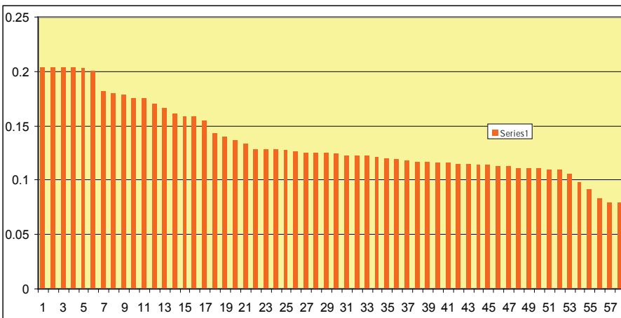
58 transistor sorted by decreasing Ice
