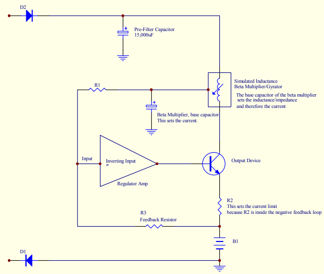
Simplified Diagram of the "Linear Amp Regulator, To Clearly show this ia a class A amplifier
