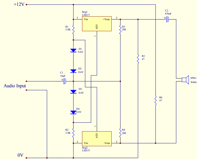
Complimentary Regulator Phase Splitter Audio Amp Ver.2
