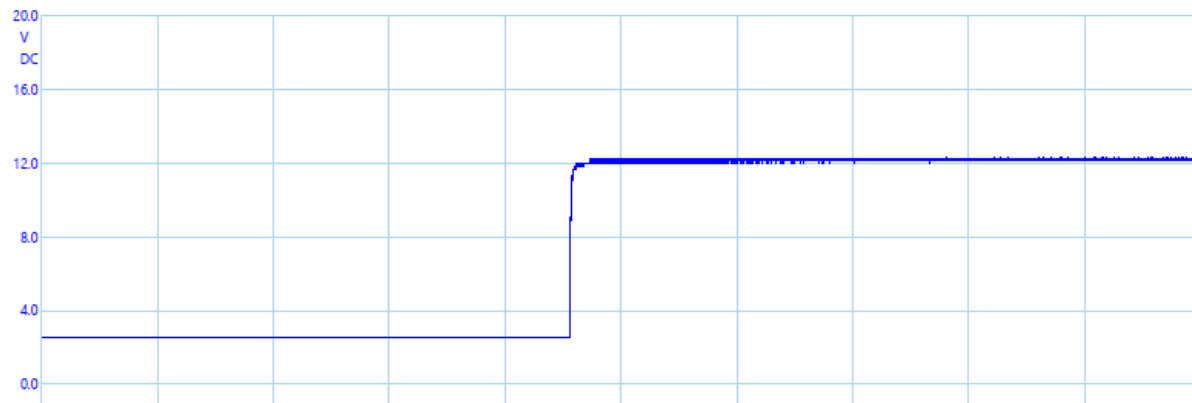
Capacitor voltage DURING connecting secondary battery
