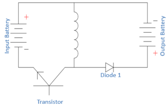
Radiant mode simplified
