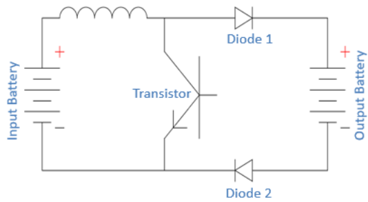
Common ground / Generator mode simplified
