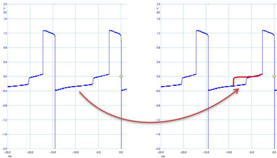
Attachment: Scope shot over one of the main coil windings
