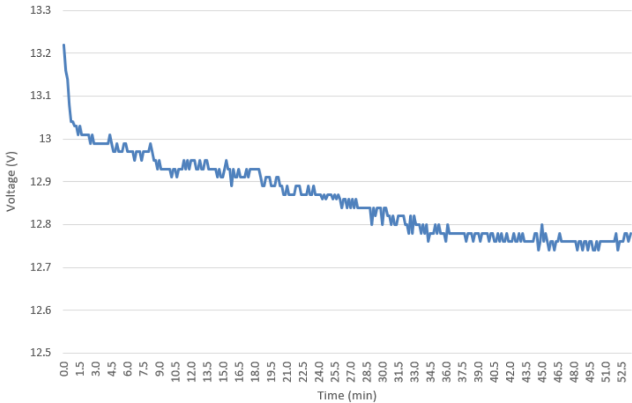
D12 2020-jan-04 16:31 Discharge 12Ah battery @ +/- C20 rate
