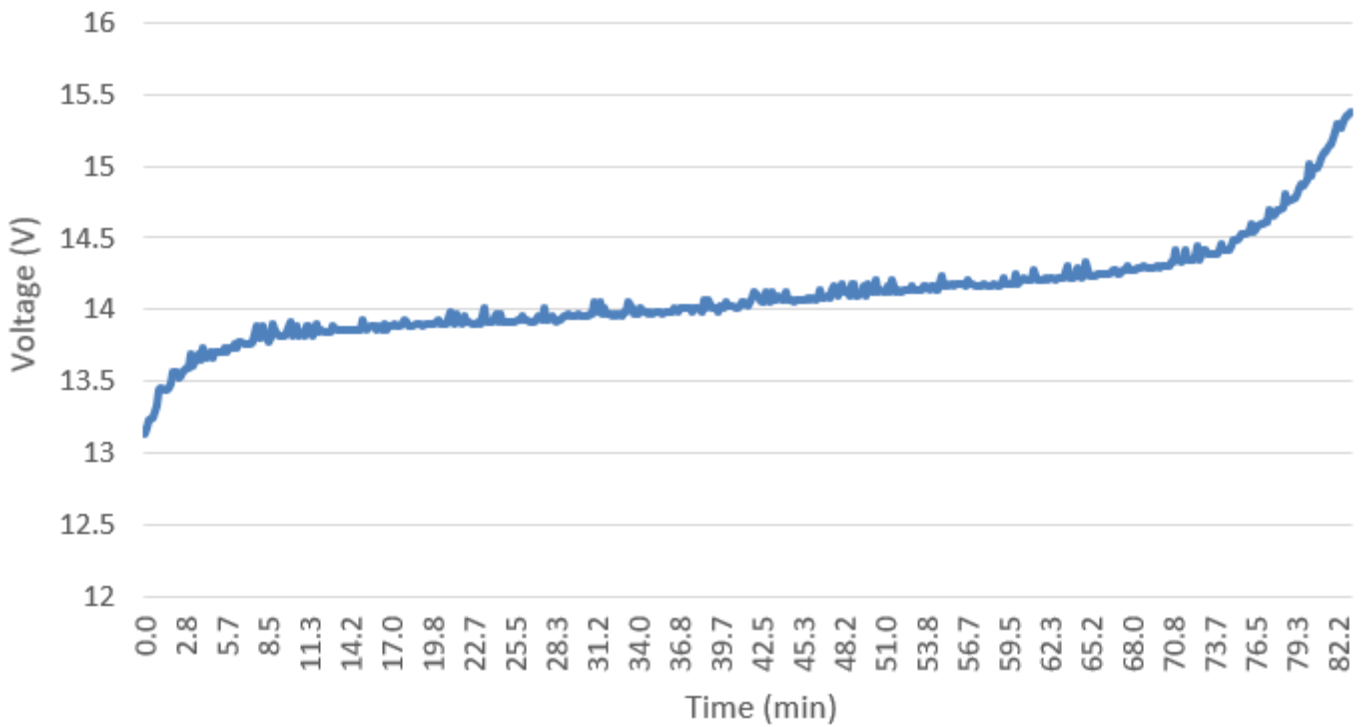
C12 2020-jan-04 18:33 Charge 12Ah battery
