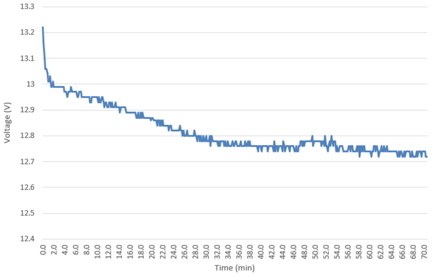
D10 2020-jan-03 14:40 Discharge 12Ah battery @ +/- C20 rate
