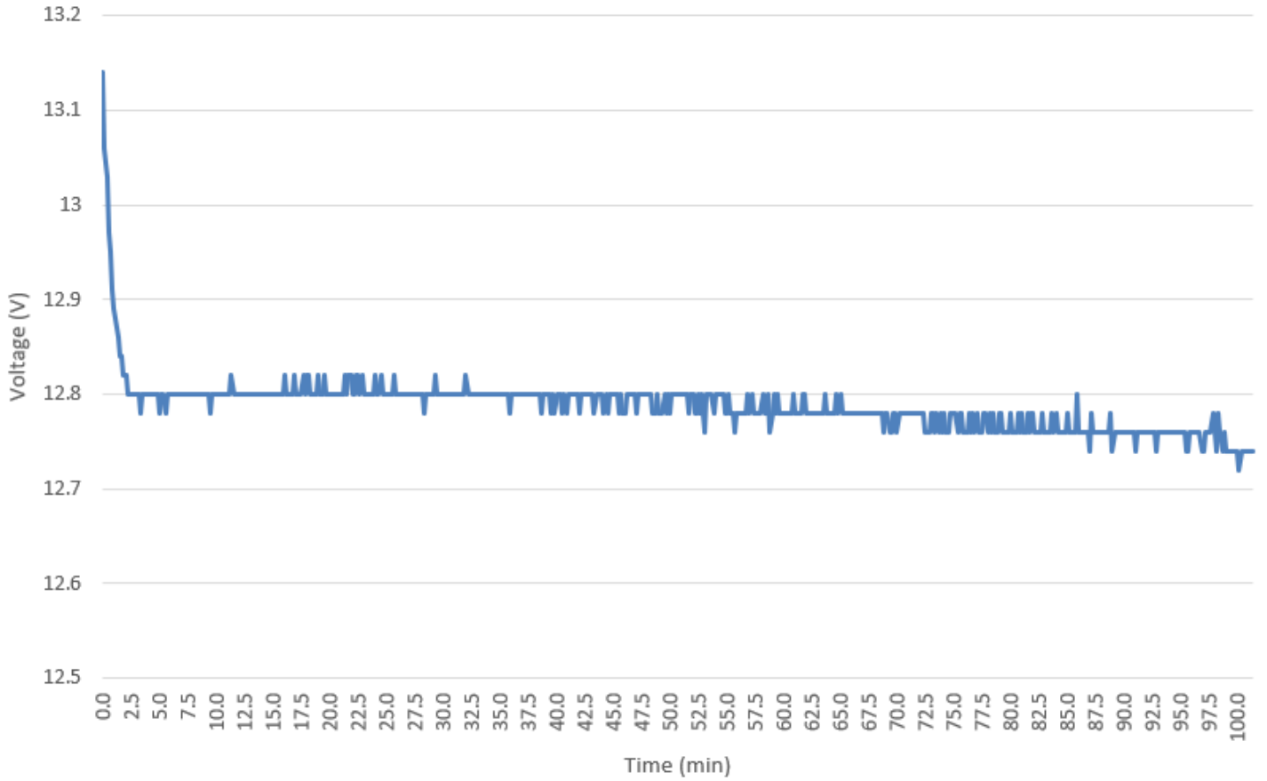
D8 2020-jan-01 17:27 Discharge 12Ah battery @ +/- C20 rate
