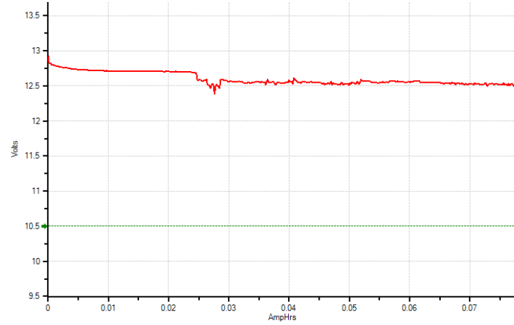
Battery A: too low resting voltage 12.68V
